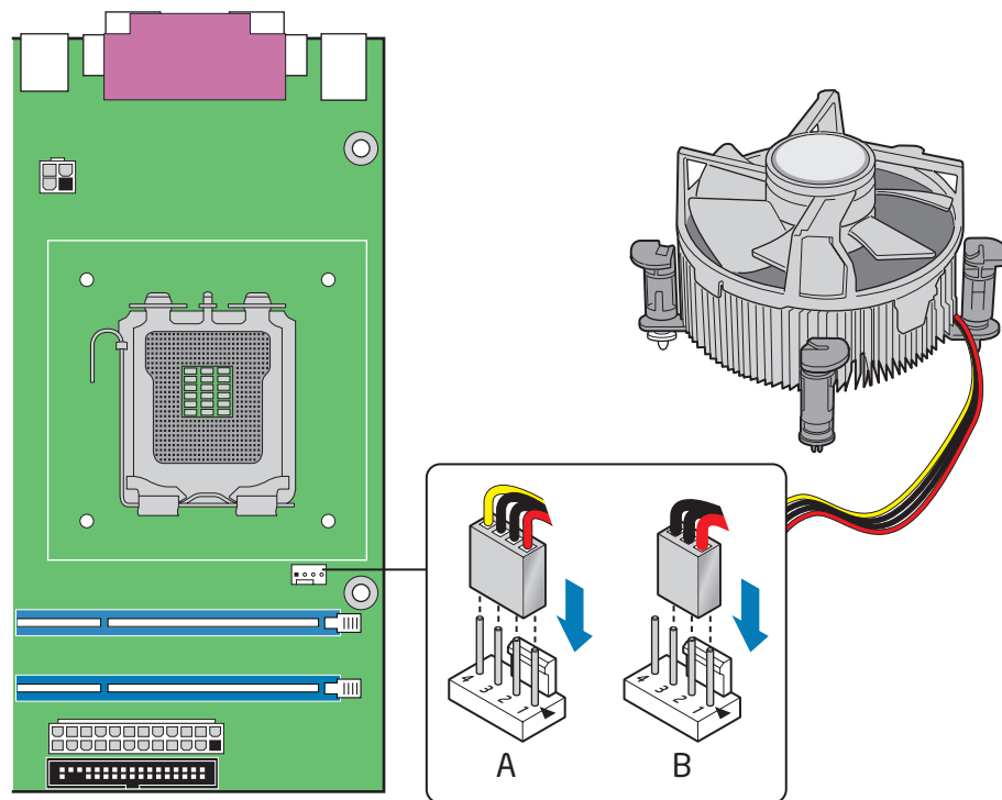
Figure 12. Connecting the Processor Fan Heat Sink Cable to the Processor Fan Header
